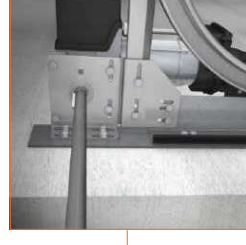
Plastics profile behind frame PVC wall partition equipped with comriband between frame and wall are separate parts for easy and efficient maintenance.
